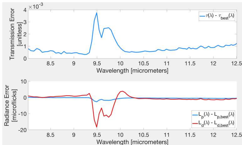
Figure 7. Spectral differences between transmission, path radiance, and downwelling radiance and truth for the Model 6 atmosphere and best (288 \text{ K}, 7800 \text{ ppmv}) pair.
