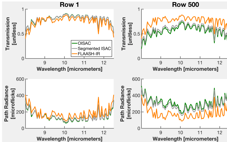
Figure 18. Transmission and path radiance for the three AC techniques for the first and last rows the Model 6 synthetic scene.
