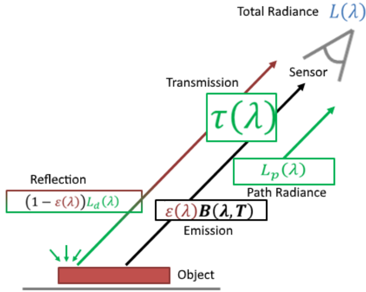
Figure 2. Pictorial representation of the sensed radiance model. Total radiance at the sensor, L(\lambda) , is a combination of path radiance contributions, L_p(\lambda) , emissions, and reflections.
