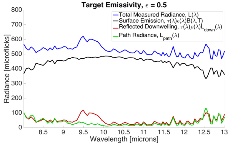
Figure 3. Example of relative contributions to the total sensed radiance for a \epsilon = 0.5 graybody. The summation of the surface emission (black), reflected downwelling (red), and path radiance (green) terms yields the total radiance (blue).
